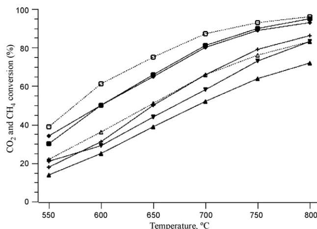
Fig. 2. Dry reforming tests with diluted reactants. CH_4 conversions for (◆) Ni/Ce_2Zr_2 (imp); (+) NiCoCe_2Zr_{1.51} (sg); (▲) NiCe_{0.6}Zr_{2.97} (sg); (□) NiCe_2Zr_{1.51} (sg) and (···) NiRhCe_2Zr_{1.51} (sg). CO_2 conversions are depicted with dotted lines for the most and the least active samples: (□) NiRhCe_2Zr_{1.51} and (Δ) NiCe_{0.6}Zr_{2.97} (sg). Reaction conditions: CH_4/CO_2/Ar = 10/10/80 ; total space velocity: 30\text{ L h}^{-1}\text{ g}^{-1} .
